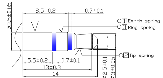
MATCHING PLUG
