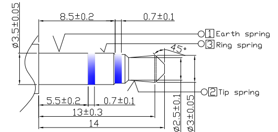
MATCHING PLUG
