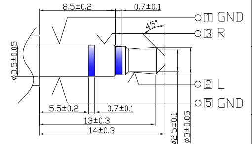
MATCHING PLUG
