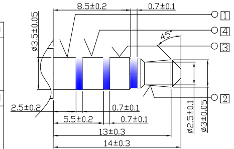
MATCHING PLUG
