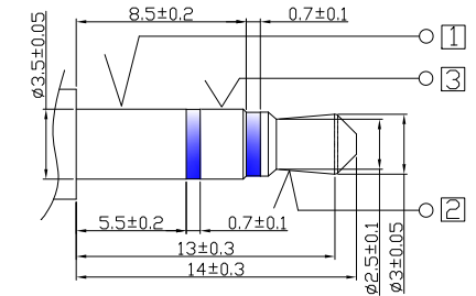
MATCHING PLUG
