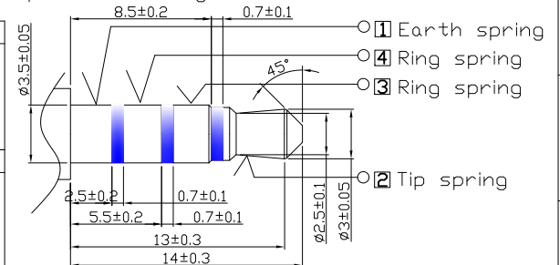
MATCHING PLUG
