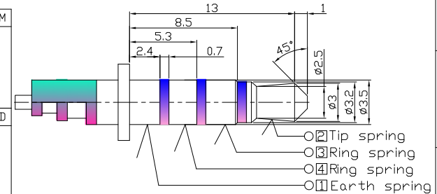
MATCHING PLUG
