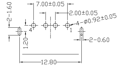
FRONT EDGE OF CONNECTOR PCB LAYOUT (T=1.60mm)
