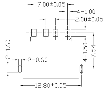
FRONT EDGE OF CONNECTOR PCB LAYOUT (T=1.60mm)
