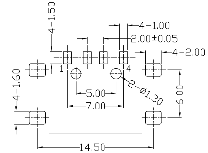
FRONT EDGE OF CONNECTOR PCB LAYOUT
