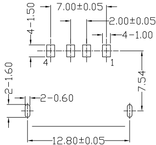
FRONT EDGE OF CONNECTOR PCB LAYOUT (T=1.60mm)
