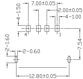
FRONT EDGE OF CONNECTOR PCB LAYOUT (T=1.60mm)
