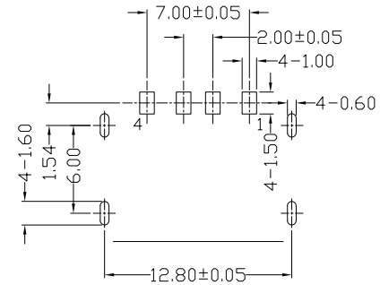
FRONT EDGE OF CONNECTOR PCB LAYOUT (T=1.60mm)
