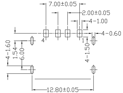
FRONT EDGE OF CONNECTOR PCB LAYOUT (T=1.60mm)
