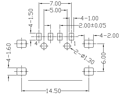
FRONT EDGE OF CONNECTOR PCB LAYOUT
