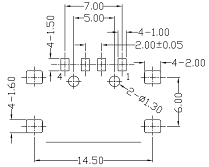
FRONT EDGE OF CONNECTOR PCB LAYOUT
