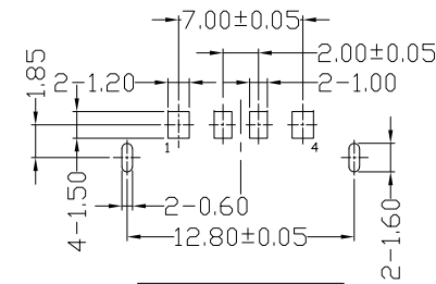
FRONT EDGE OF CONNECTOR PCB LAYOUT (T=1.60mm)
